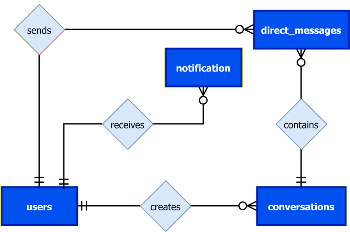
Figure 22: Messaging & Notifications ERD
