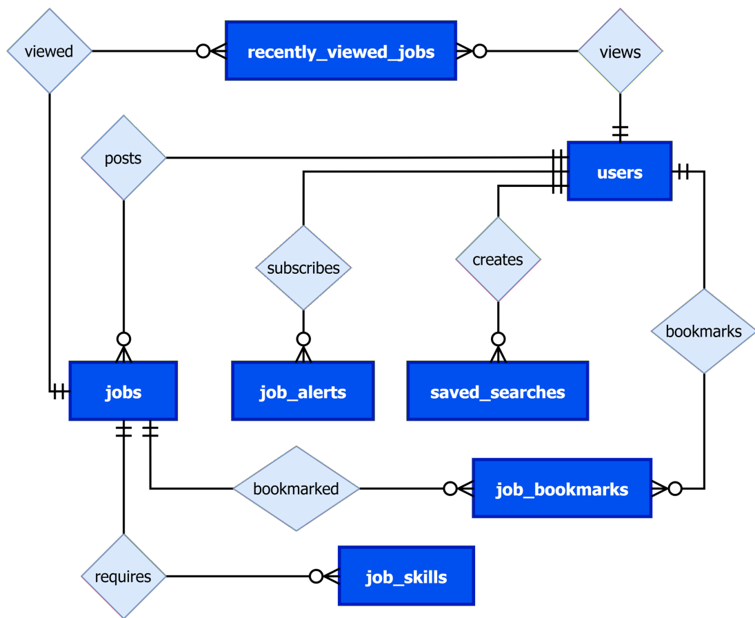
Figure 16: Job Posting & Discovery ERD
